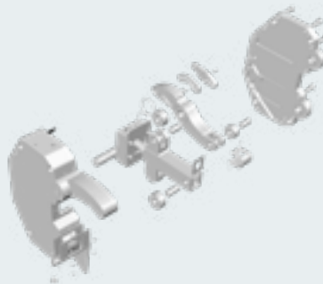
Component Steady rest 73 kg
