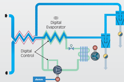
Figure 2 - Digital Evaporator Refrigeration Control
