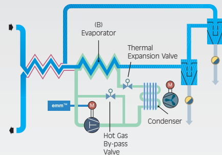
Figure 3 - Hot Gas Bypass Valve Refrigeration Control
