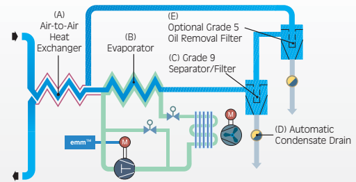
Figure 1 - Air Drying Circuit
